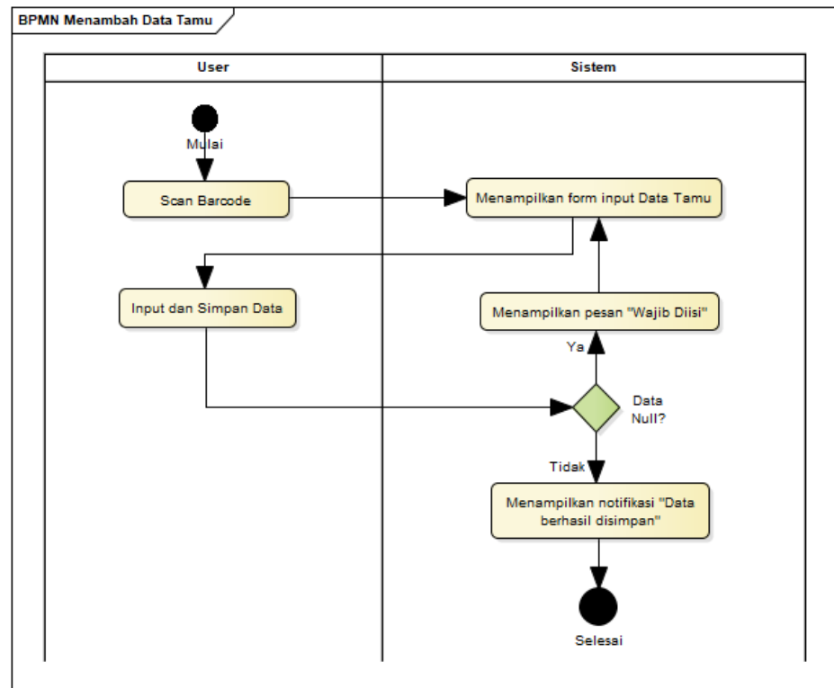
Gambar 4. Diagram Activity Menambah Data Tamu (User)
