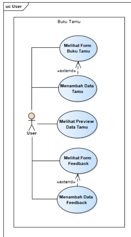
Gambar 2. Usecase Diagram (User)
