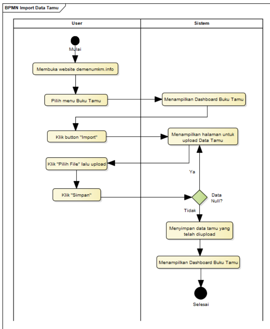
Gambar 8. Diagram Activity Import Data Tamu (Admin)
